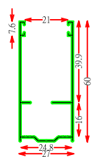
GU6027 ANTIVENTO
